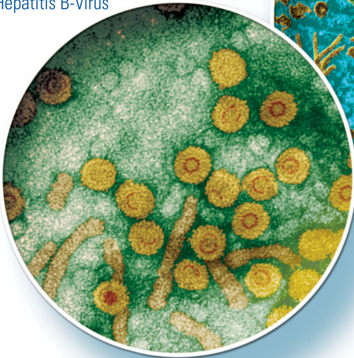
Hepatitis B-Virus
