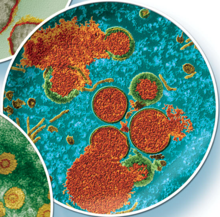
Vacciniavirus
